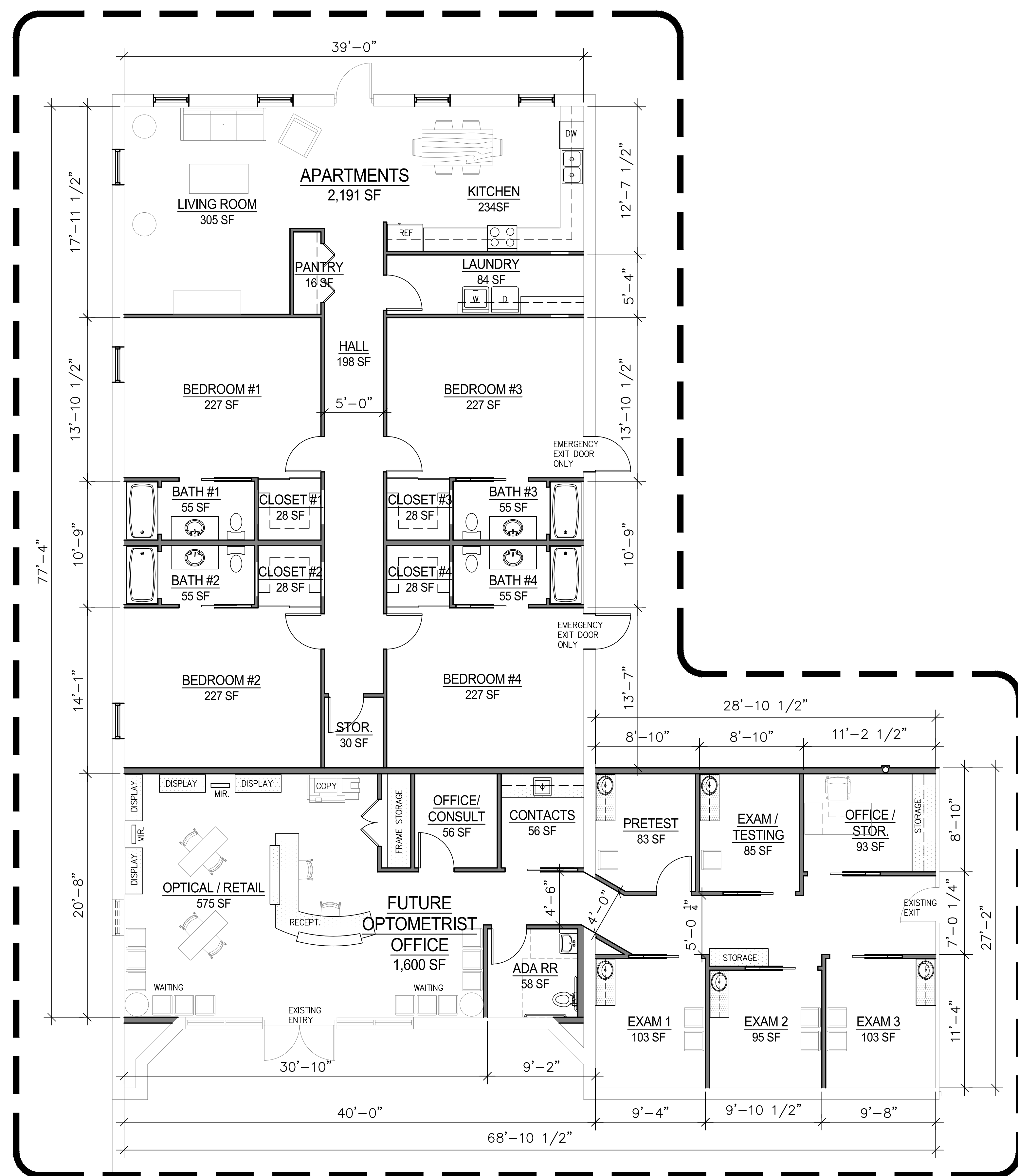
RFP - PHASE 1 LAYOUT 3/16" = 1'-0"
