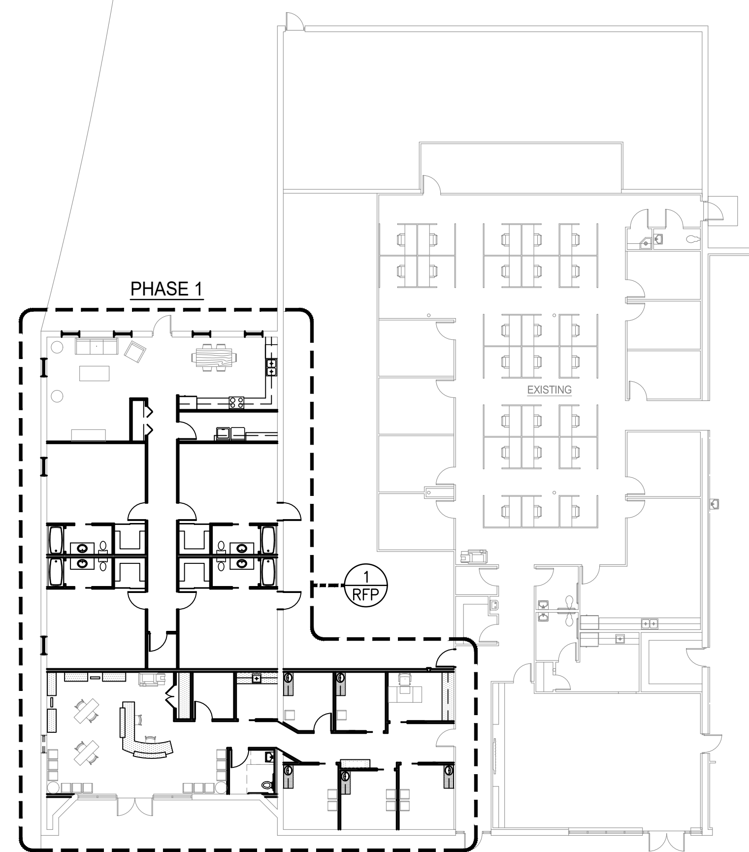
KEYED PLAN 1/16" = 1'-0"
